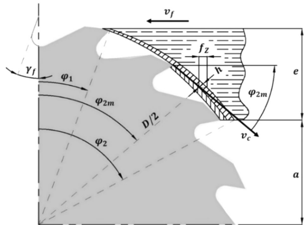
Fig. 4 Sawing kinematics of circular saw cutting
