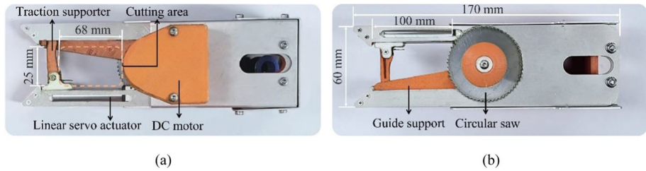
Fig. 5 The proposed cutting module: a top view and b bottom view
